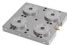
Zero position
